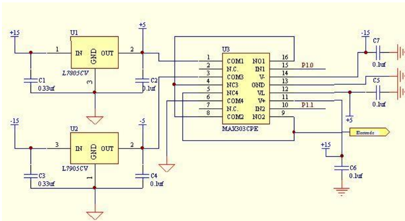
Fig. 5. Bipolar pulse excitation circuit
