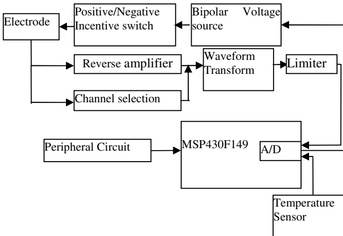
Fig. 4. Structure of the Intelligence Electrode Conductivity Meter
