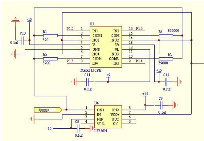
Fig. 6. Range Switching and Amplifier Circuit
