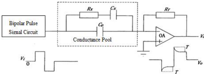
Fig. 3. EC Measurement based on Bipolar Pulse Excitation
