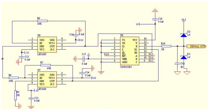
Fig. 7. Waveform Transformation Circuit
