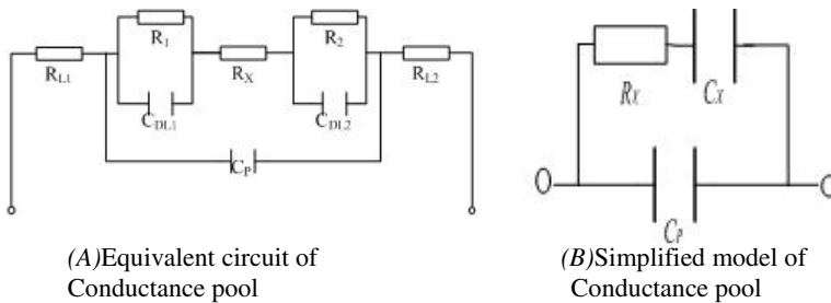
Fig. 1. Conductance pool and its Equivalent circuit
