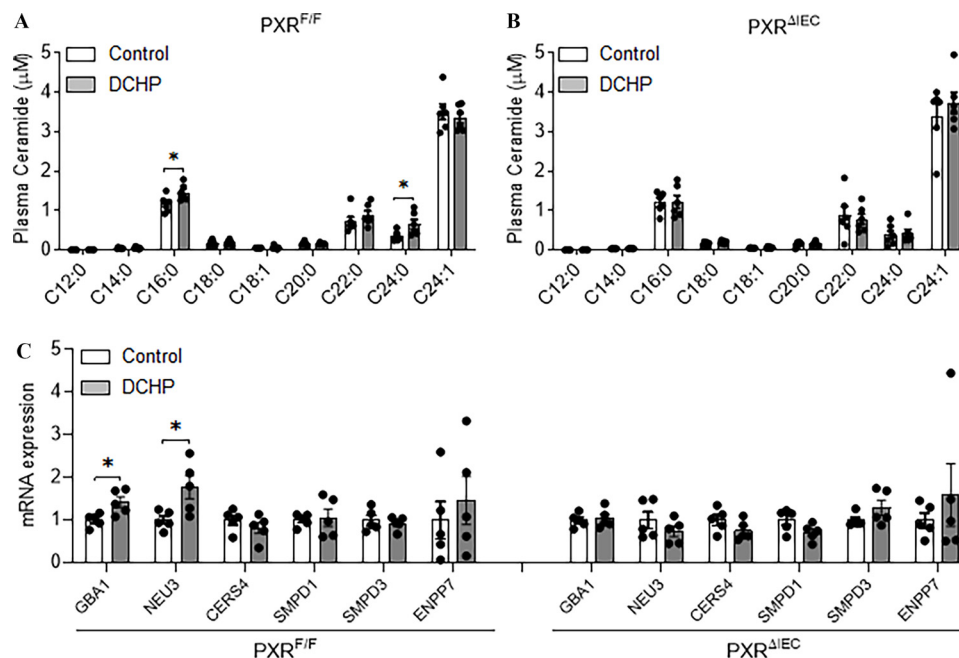
Figure 6. The impact of DCHP exposure on circulating ceramide levels and ceramide-synthesis-related gene expression in PXR^{F/F} and PXR^{\Delta IEC} mice. Eight-wk-old male PXR^{F/F} and PXR^{\Delta IEC} littermates were treated with vehicle control or 10 mg/kg BW per day of DCHP daily by oral gavage for 7 d. Plasma ceramide levels of (A) PXR^{F/F} and (B) PXR^{\Delta IEC} mice were measured by LC-MS/MS ( n = 6 , two-sample, two-tailed Student's t -test, *, p < 0.05 ). (C) Intestinal expression of ceramide-synthesis-related genes were measured by qPCR ( n = 5 , two-sample, two-tailed Student's t -test, *, p < 0.05 ). The numerical data corresponding to this figure are shown in Tables S15–S16. Results represent mean values. Error bars represent \pm SEM. Note: BW, body weight; CERS4, ceramide synthase 4; DCHP, dicyclohexyl phthalate; ENPP1, ectonucleotide pyrophosphatase/phosphodiesterase 1; GBA1, glucosylceramidase beta 1; LC-MS/MS, liquid chromatography–tandem mass spectrometry; NEU3, neuraminidase 3; PXR^{\Delta IEC} , intestinal epithelial cell-specific pregnane X receptor deficient; PXR^{F/F} , pregnane X receptor floxed; SMPD1, sphingomyelin Phosphodiesterase 1; SMPD3, sphingomyelin Phosphodiesterase 3; qPCR, quantitative polymerase chain reaction; SEM, standard error of the mean.
