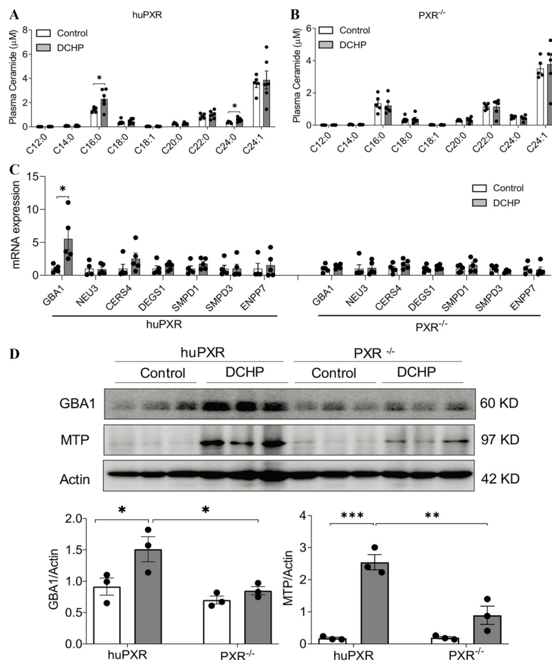
Figure 8. The impact of DCHP exposure circulating ceramide levels and ceramide-synthesis-related gene expression in PXR-humanized (huPXR) mice. Eight-wk-old male huPXR and PXR -/- littermates were treated with 10 mg/kg BW per day of DCHP or vehicle control daily by oral gavage for 7 d. Plasma ceramide levels of (A) huPXR and (B) PXR -/- mice were measured by LC-MS/MS. ( n = 5-6 , two-sample, two-tailed Student's t -test, ^*p < 0.05 ). (C) Intestinal expression of ceramide-synthesis-related genes were measured by qPCR ( n = 4-5 , two-sample, two-tailed Student's t -test, ^*p < 0.05 ). (D) Immunoblotting of GBA1, MTP, and Actin proteins in the intestine of huPXR and PXR -/- mice. The densitometry analyses of the protein bands were shown below the immunoblotting panel ( n = 3 , two-way ANOVA, Bonferroni multiple comparisons test for multiple comparisons, ^*p < 0.05 , ^{**}p < 0.01 , and ^{***}p < 0.001 ). The numerical data corresponding to this figure are shown in Tables S19–S21. Results represent mean values. Error bars represent \pm SEM. Note: ANOVA, analysis of variance; DCHP, dicyclohexyl phthalate; GBA1, glucosylceramidase beta 1; LC-MS/MS, liquid chromatography–tandem mass spectrometry; MTP, microsomal triglyceride transfer protein; PXR -/- , pregnane X receptor deficient; qPCR, quantitative polymerase chain reaction; SEM, standard error of the mean.
